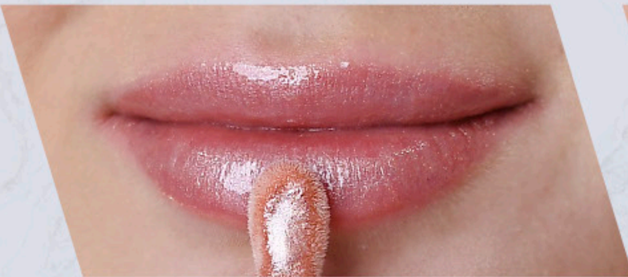
3 - SUPERNOVA
